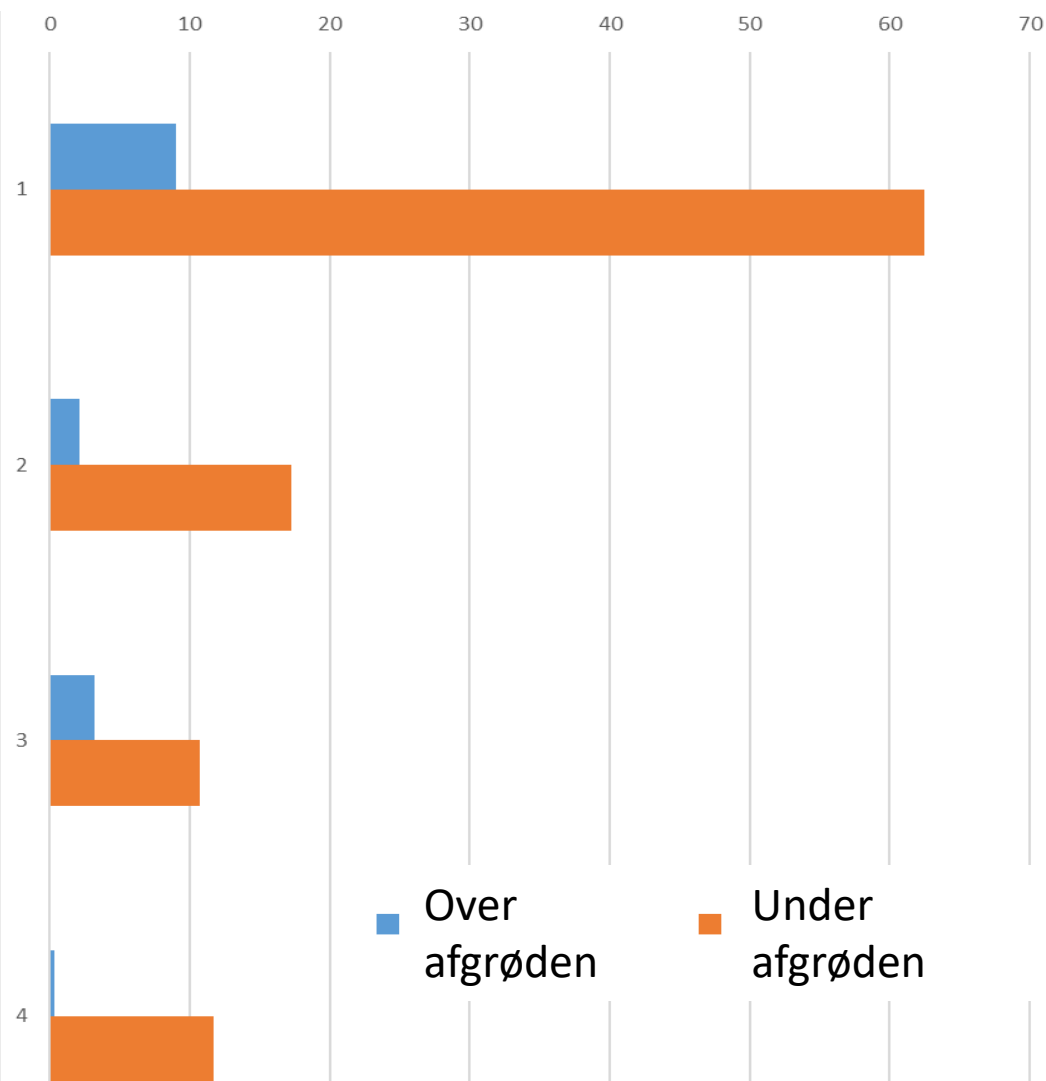
Total weed coverage ultimo July
